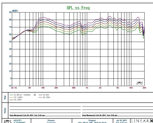
Frequency Response
